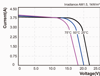
I-V Curves of PV module SY-S65W at various cell temperatures
