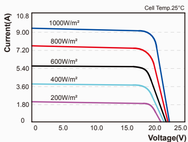
I-V Curves of PV module SY-S160W
