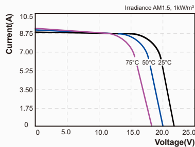
I-V Curves of PV module SY-S150W at various cell temperatures
