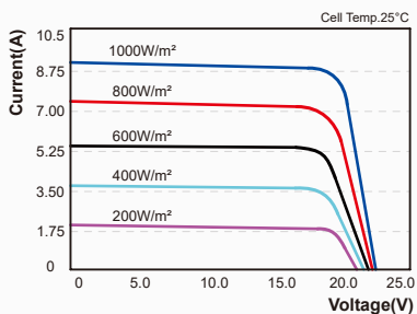
I-V Curves of PV module SY-S150W
