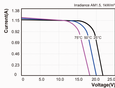
I-V Curves of PV module SY-M20W at various cell temperatures
