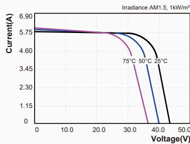
I-V Curves of PV module SY-M200W at various cell temperatures
