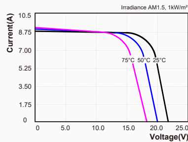
I-V Curves of PV module SY-M150W at various cell temperatures
