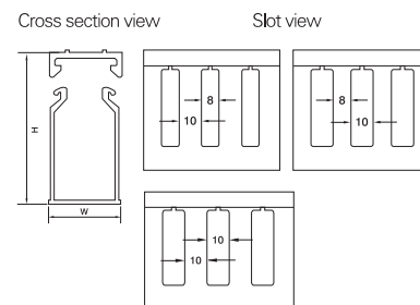
Single row bottom hole view ( W < 80 )
