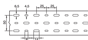
Triple rows bottom hole view ( W \geq 80 )
