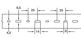
Single row bottom hole view ( W < 80 )
