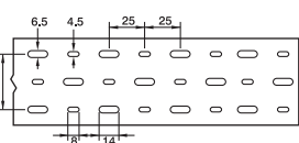
Triple rows bottom hole view ( W ≥ 80 )
